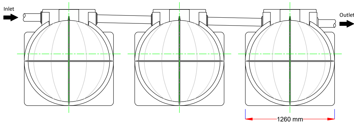
Side elevation
