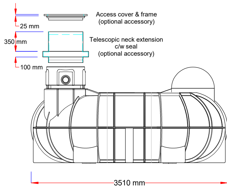
SIDE ELEVATION
