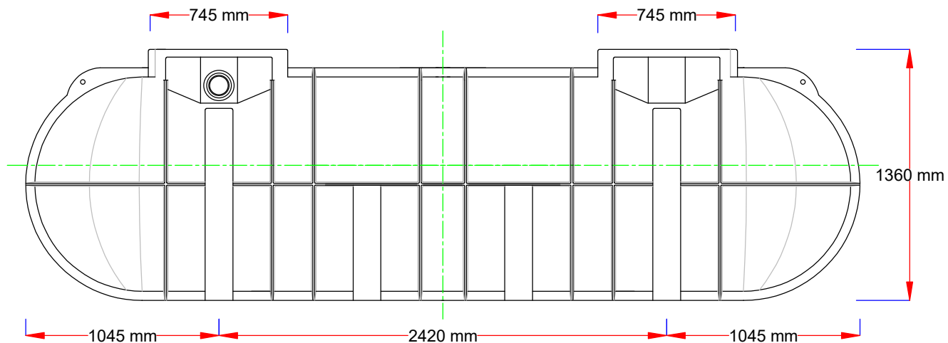
Side elevation
