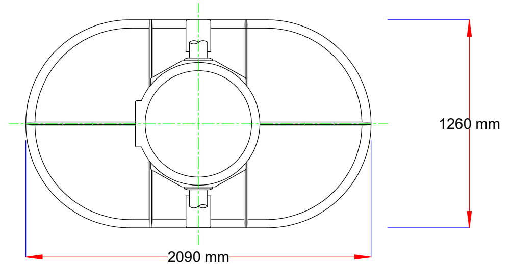
Plan view
