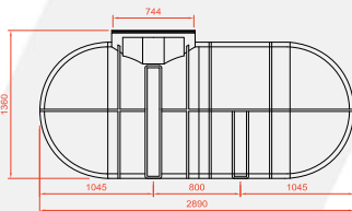
SIDE ELEVATION
