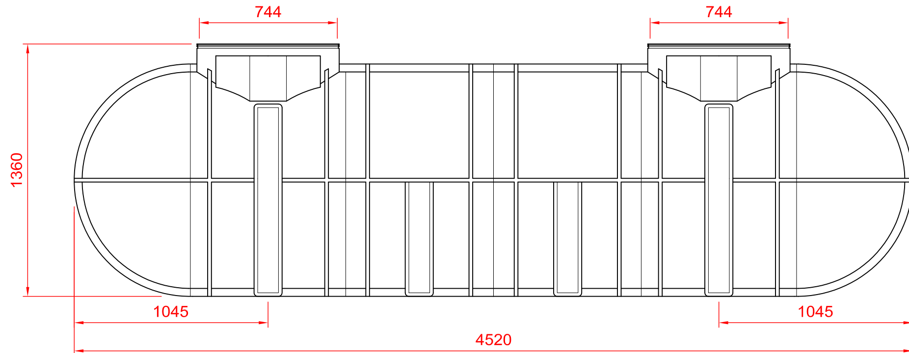
SIDE ELEVATION
