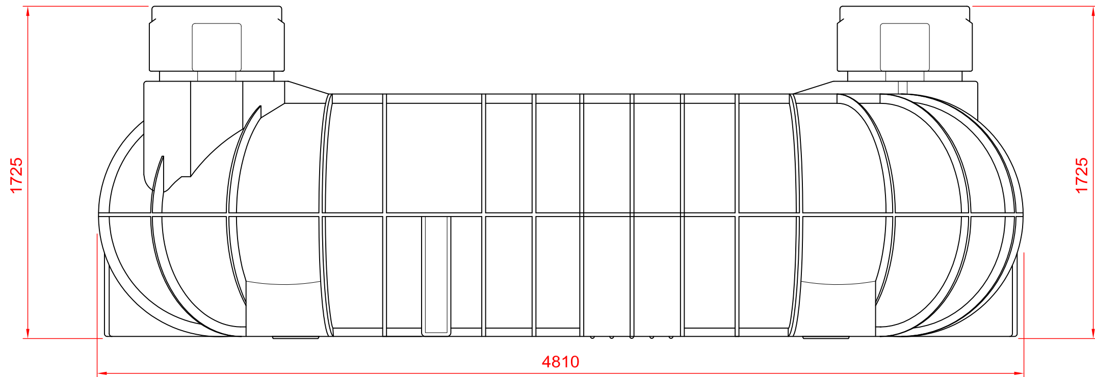
SIDE ELEVATION
